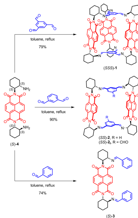
Scheme 1. Synthesis of 1–3 15
