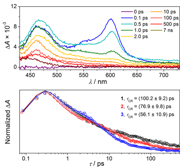
Figure 3. Femtosecond transient absorption spectra of 1 in CH 2 Cl 2 at 298 K following a 350 nm laser pulse (0.6 μJ/pulse) excitation (top) and kinetic traces (470 nm) with associated fit (see text) for 1–3 (bottom). Lifetimes of charge recombination ( \tau_{\text{CR}} ) are shown.
